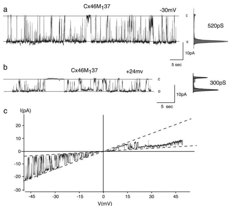
FIGURE 5 Single-channel currents in membrane patches excised from oocytes expressing Cx46M 1 37 at negative (a) potential, positive (b) potential, and during voltage ramps from +50 to −50 mV (c). All-point amplitude histograms and single-channel conductance at negative and positive potentials are shown beside the corresponding current traces.
