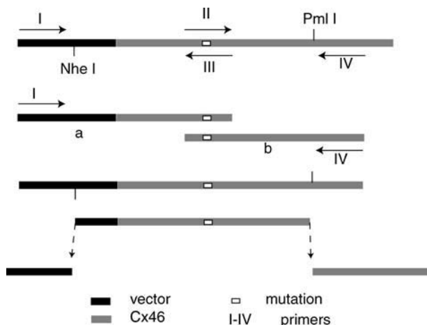
FIGURE 1 Construction of the Cx46 mutants: Cx46M 1 32, Cx46M 1 37, and Cx46L35G. A replacement cassette flanked by two restriction enzyme sites, Nhe I and Pml I, was generated by PCR.
